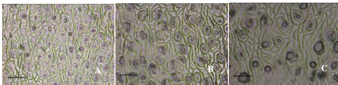
Figure 6. Stomata on lower leaf epidermis of pummelo 'Nambangan' shoots from in vitro colchicine treatment and control: A. Diploid (control), B. Mixoploid, and C. Tetraploid (bar = 50 \mu m).
