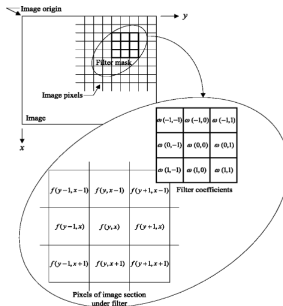
Figure 1. The mechanics of spatial filter using a 3 \times 3 mask [14]
