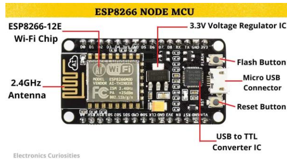
Figure 2. ESP8266 NodeMCU [26]
