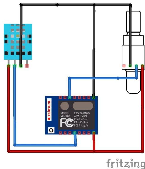
Figure 3. Hardware connection
