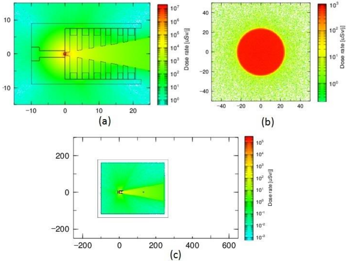
Figure 4. (a) Distribution of kerma dose rate on Al collimator with ^{241}\text{Am} source, (b) Field size of beam at 100 cm, dan (c) Distribution af air kerma in the room.
