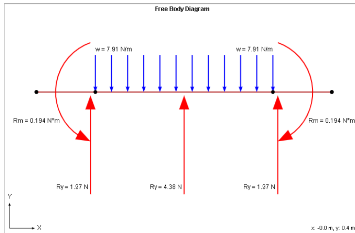
Figure 5. Simulation Results of Continuous Loading of Flange's Spokes
