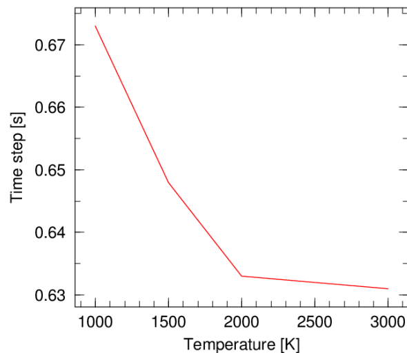
Figure 7. Effect of temperature on corium flow time
