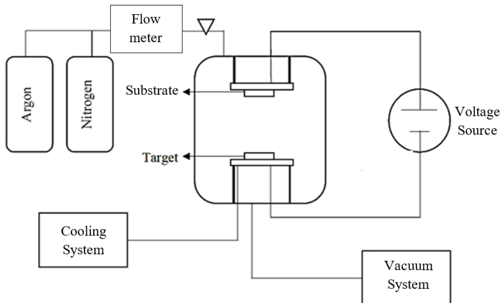
Figure 1. Schematic of DC Sputtering Device [18]
