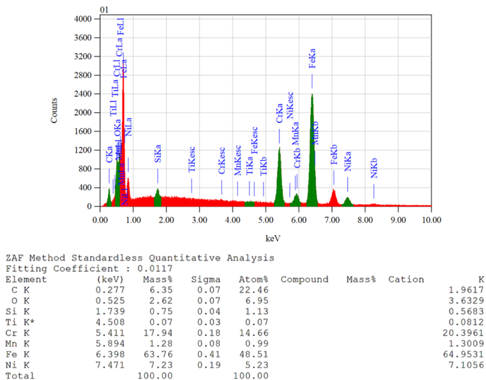
Figure 7. EDX micrograph of 316L stainless steel material after the DC sputtering process
