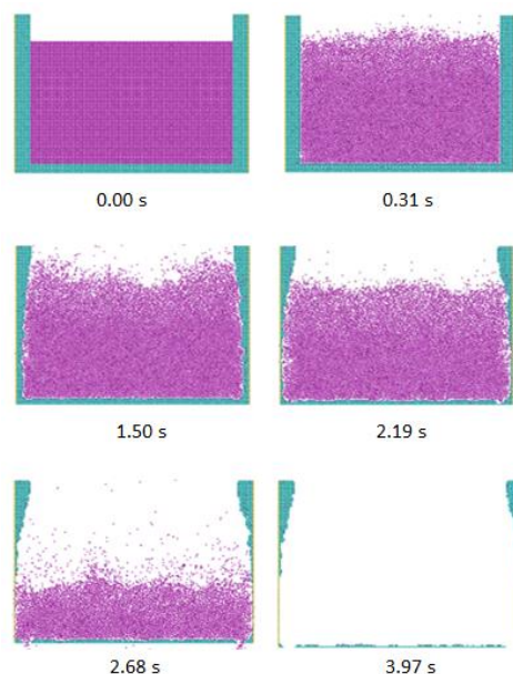
Figure. 7. Diffusion pattern of molten uranium into the wall of penetration tube.
