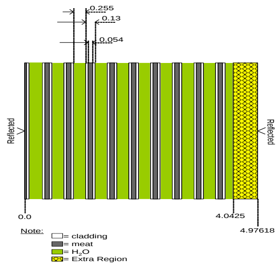
Figure 4. Fuel cell model [15].
