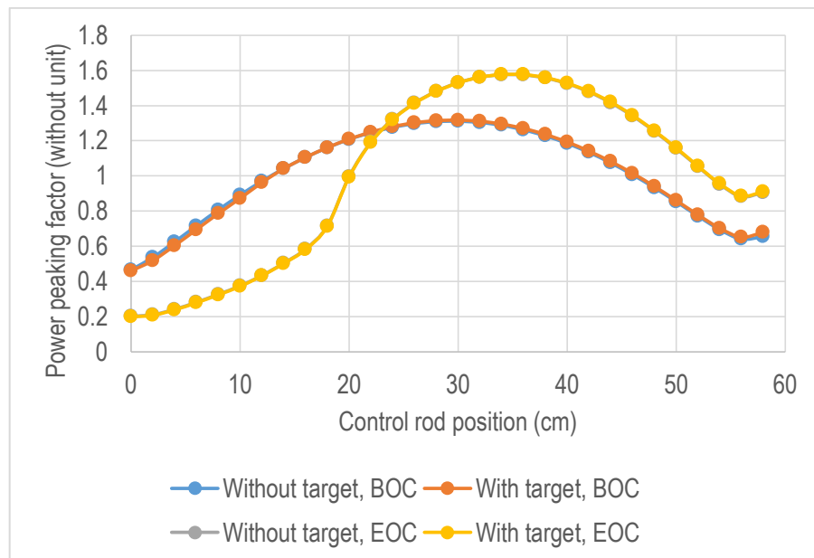
Fig. 5. The axial distribution of power peaking factor without dan with target at CIP
