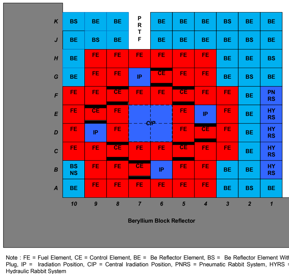
Fig. 1. Equilibrium silicide core of RSG-GAS reactor
