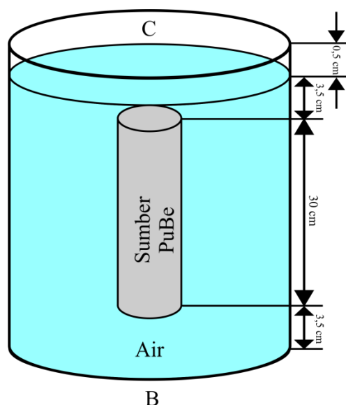
Gambar 4. Container Air Tampak Samping.
