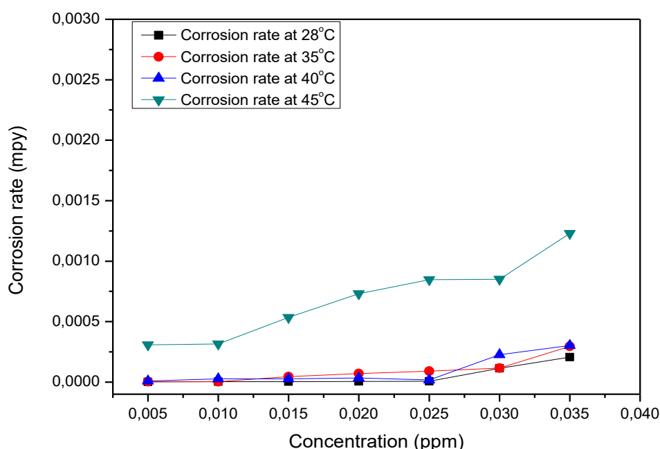
Figure 2. AlMg 2 corrosion rate in various NaCl concentrations at various temperatures in demineralized water with pH 6.7 and conductivity 0.4 \mu S/cm
