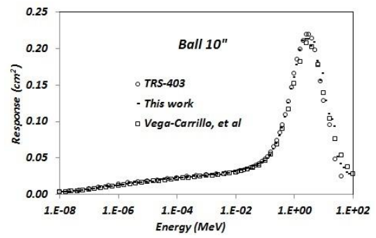
Figure 10. Neutron response function for BSS 10"
