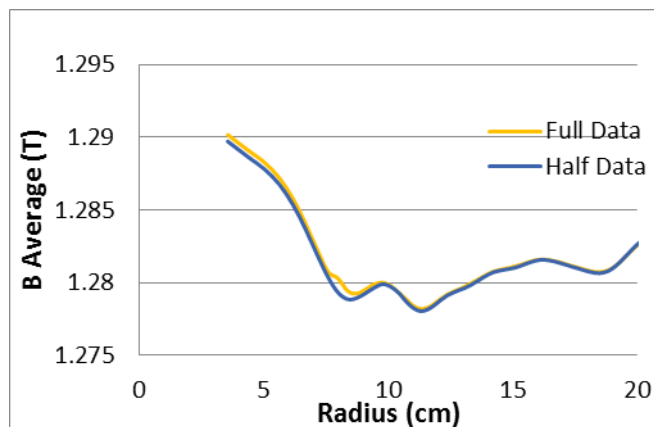
Fig. 9. Comparison of the magnetic field average calculation from a full data and a half data
