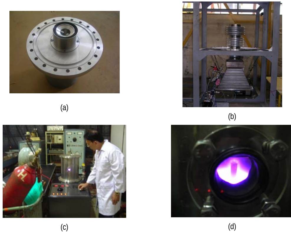
Figure 1. Some pictures of home made machine at PTAPB. Electron gun based on filament (a), Electron beam machine in construction (b), Plasma Nitriding machine (c), and an automotive component is treated by plasma nitriding machine.
