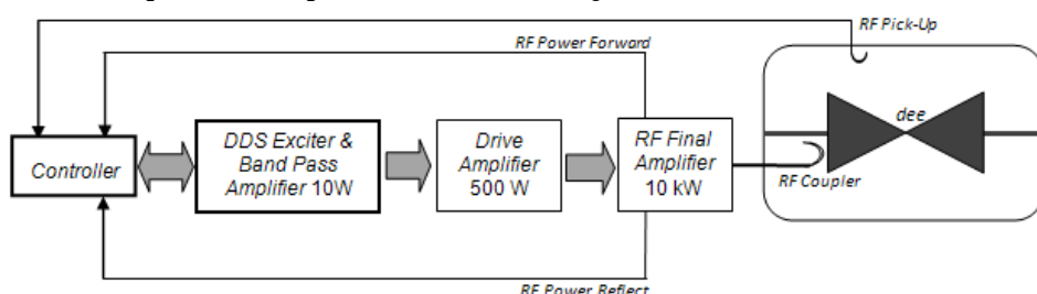
Gambar 1. Blok diagram sistem generator RF.
