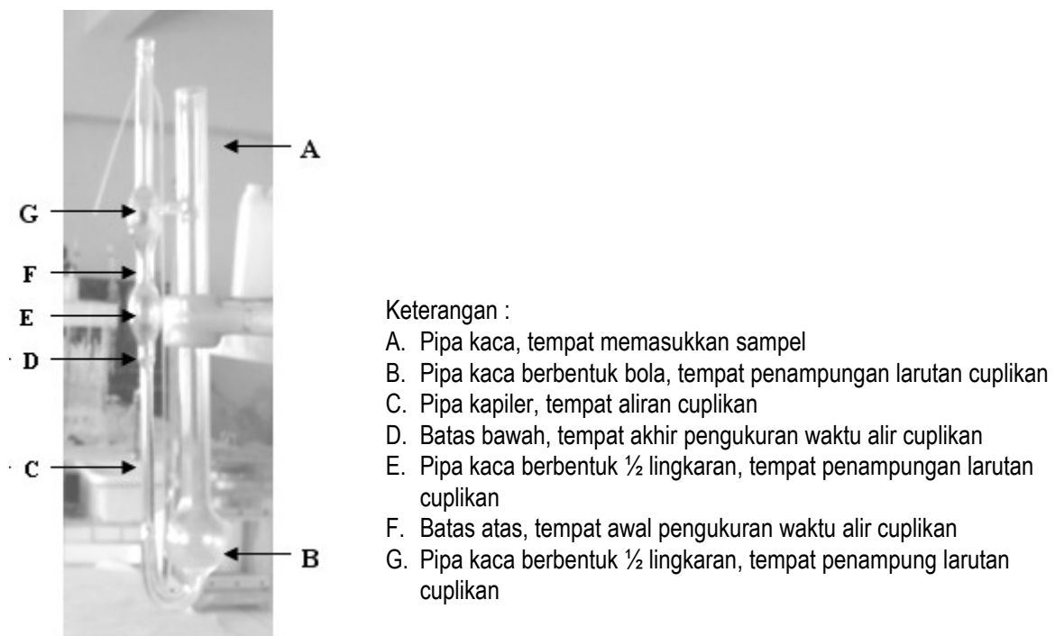
Gambar 1. Alat Viscometer Ostwald
