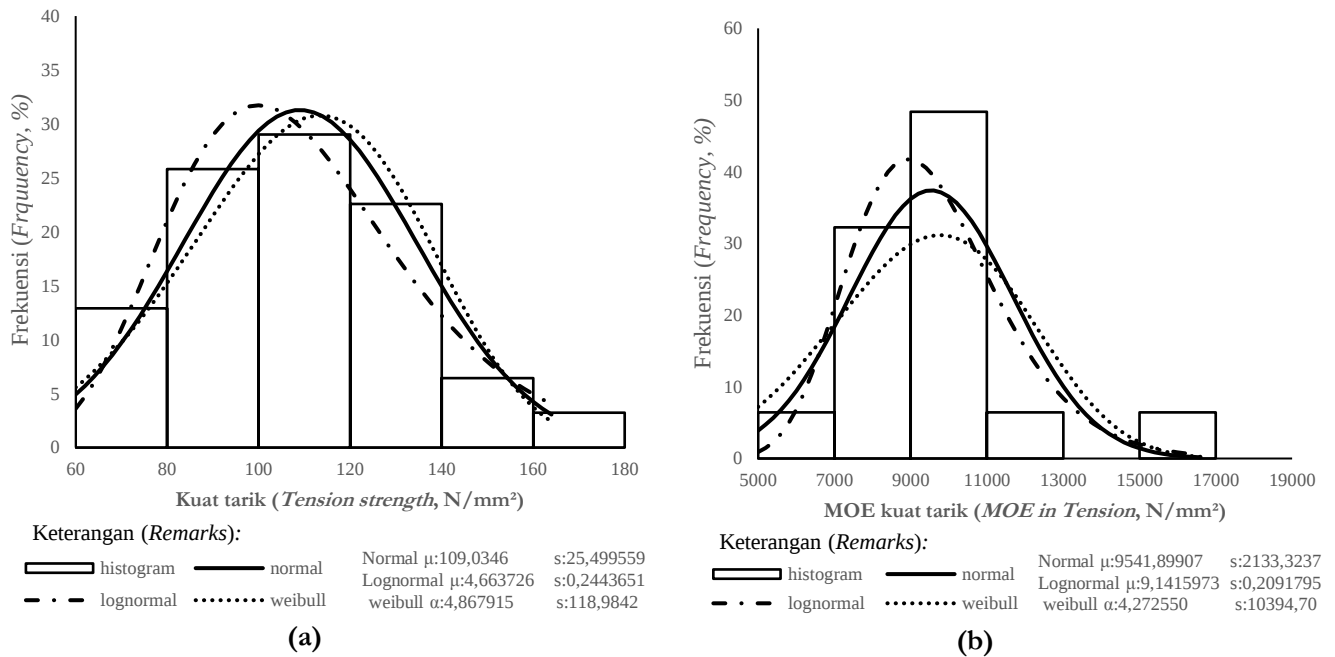
Gambar 5. Distribusi normal, lognormal, dan weibull pada data kuat tarik sejajar serat (a), dan MOE tarik sejajar serat (b) Figure 5. Normal, lognormal, and weibull distributions on the data of tension strength parallel to grain (a), and MOE in tension parallel to grain (b)
