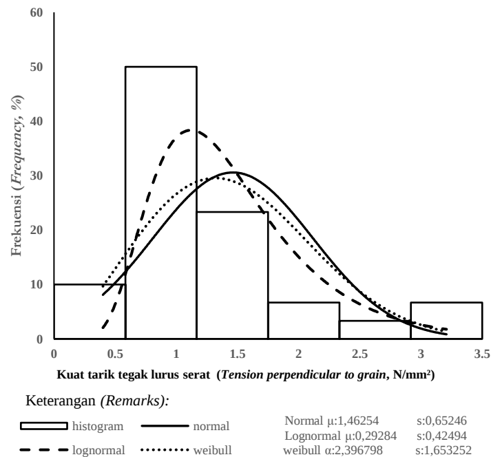
Gambar 6. Distribusi normal, lognormal, dan weibull pada data kuat tarik tegak lurus serat bambu betung Figure 6. Normal, lognormal, and weibull distributions on the data of tension perpendicular to grain of betung bamboo
