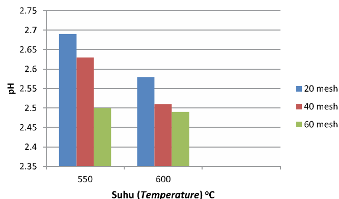
Gambar 3. pH bio-oil rumput gelagah suhu 550 – 600°C dengan ukuran 20, 40, dan 60 mesh Figure 3. Bio-oil pH content of gelagah grass at temperature 550 - 600°C and 20, 40, 60 mesh
