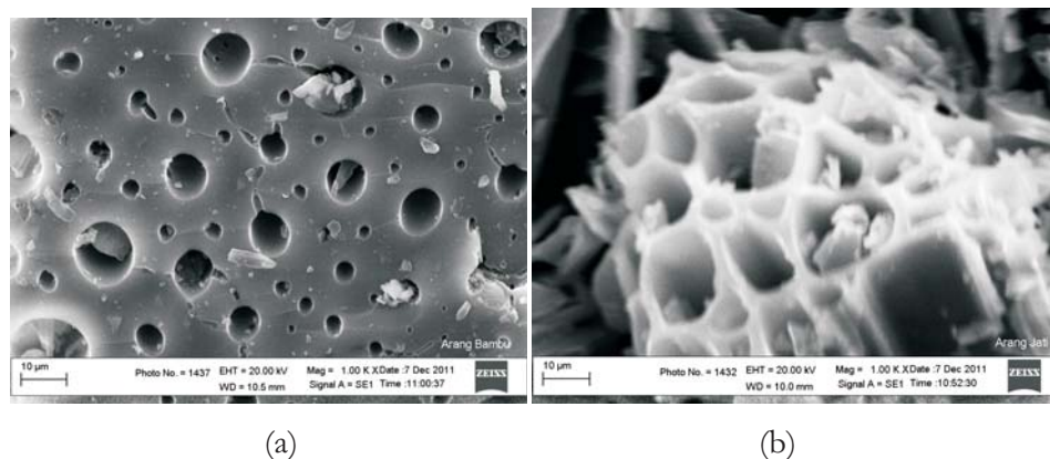
Gambar 3. Topografi pori arang dari (a) bambu dan (b) jati Figure 3. Topographic of pores from (a) bamboo and (b) teak charcoal
