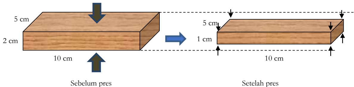
Gambar 1. Kayu jabon sebelum dipres dan setelah dipres Figure 1. Jabon wood before and after pressed
