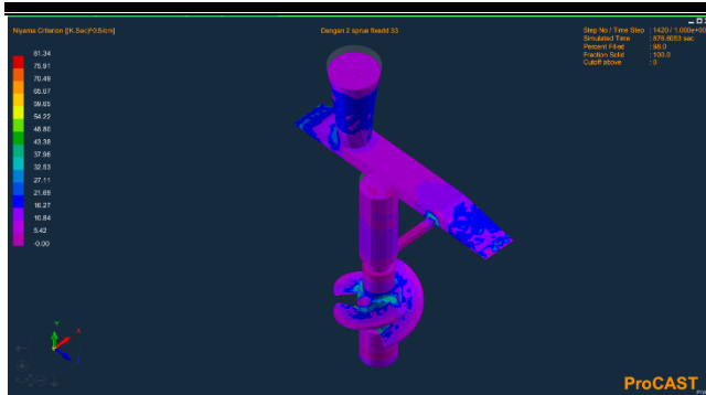
Figure 23. Niyama Criterion Design 2 Temperature 660°C
