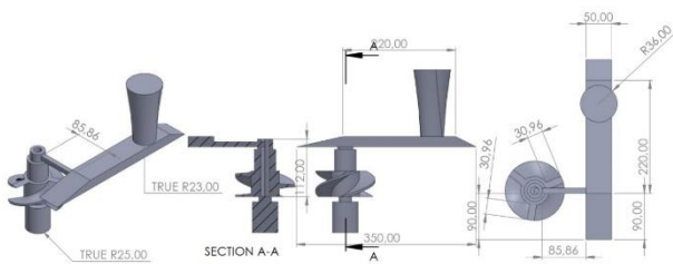
Figure 2. Design 3D Casting
