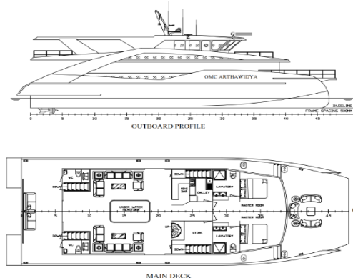
Picture 3. General Arrangement
