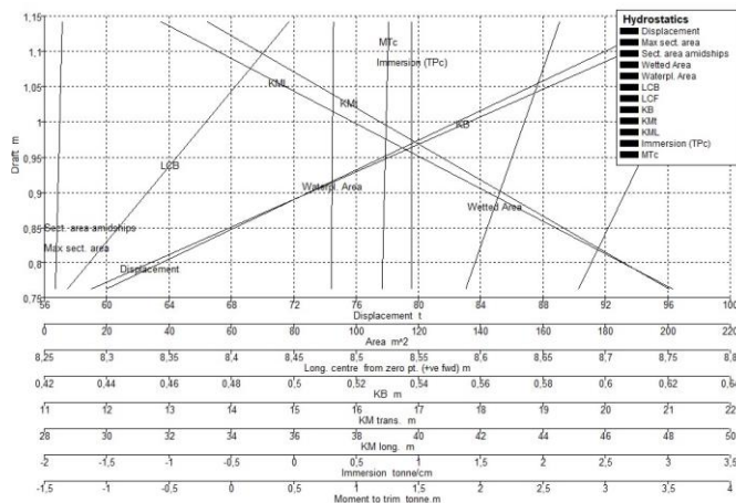
Picture 5. Hydrostatic Curve
