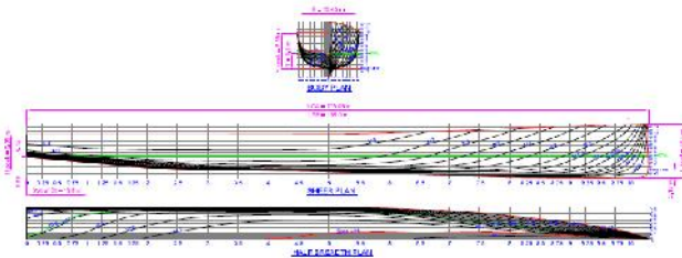
Gambar 4. Lines Plan dari Enlarge Ship Concept
