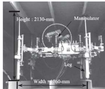
Gambar 6. IAI Rower-I, Spain (Sumber : Donghun Lee, 2014)
