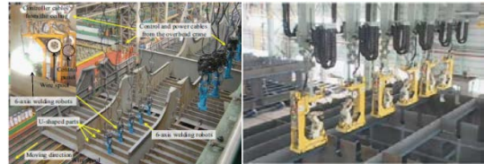
Gambar 3. 6R articulated selding robots connected to overhead crane, (Sumber : Donghun Lee, 2014)
