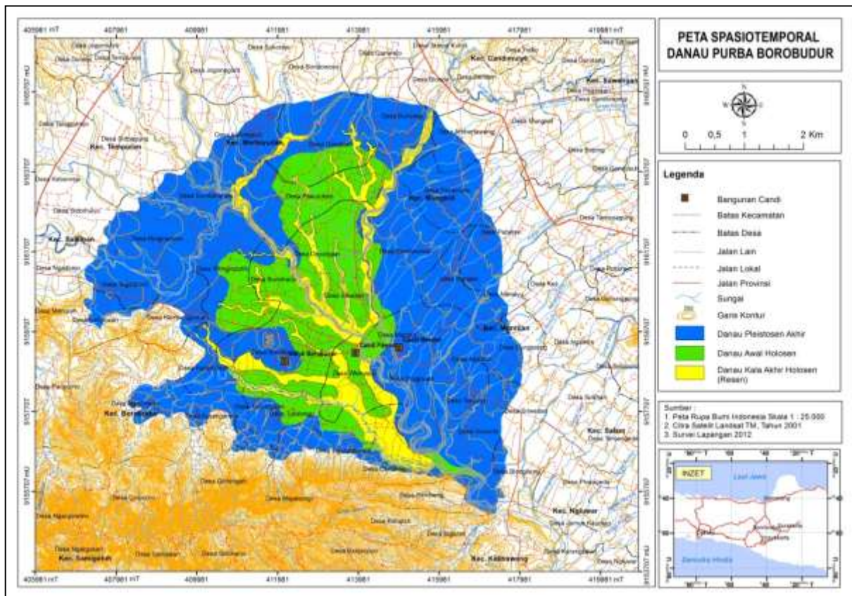
Gambar 9. Peta Spasiotemporal Danau Purba Borobudur
