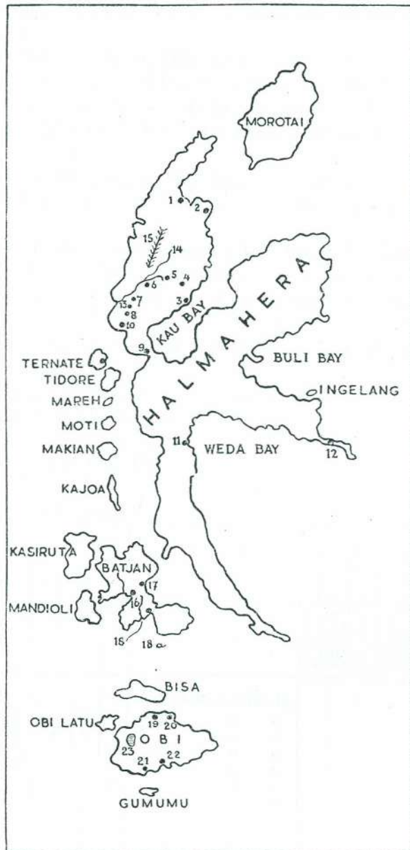
Fig. 1. Sketch Map of the North Moluccan Islands. 1 : 2,000,000.
